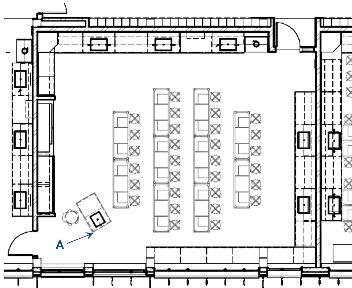
THIRD FLOOR PLAN SCIENCE ROOM
