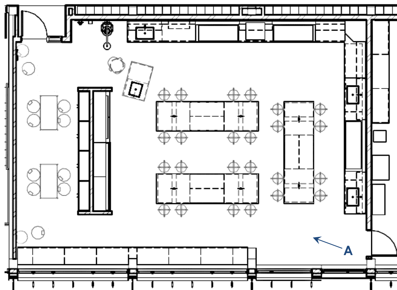
THIRD FLOOR PLAN CHEMISTRY CLASSROOMS
